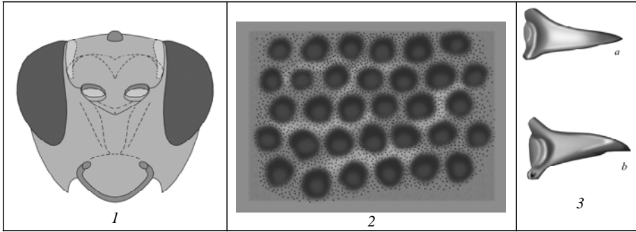
Fig. 1-3: Peculiarities of morphology of Joppocryptini: (1-2) Pseudoplatylabus uniguttatus (GRAV.): (1) contour of a head in front, (2) sculpture of mesonotum surface; (3a,b) Londokia teleji sp.n. mandible: (a) in front, (b) fronto-ventral view.
